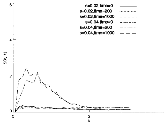
Figure 2. Temporal evolution of surfactant density structure function S(k,t) for binary water and surfactant mixtures. The figure contains results for both s = 0.02 and s = 0.04 reduced density of surfactant.
