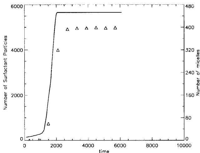
Figure 5. Amphiphile and micelle concentration as a function of the time step in the lattice-gas automaton model. The triangles are for the micelles and correspond to values on the right hand vertical axis. This case has surfactant in the system at time zero.
