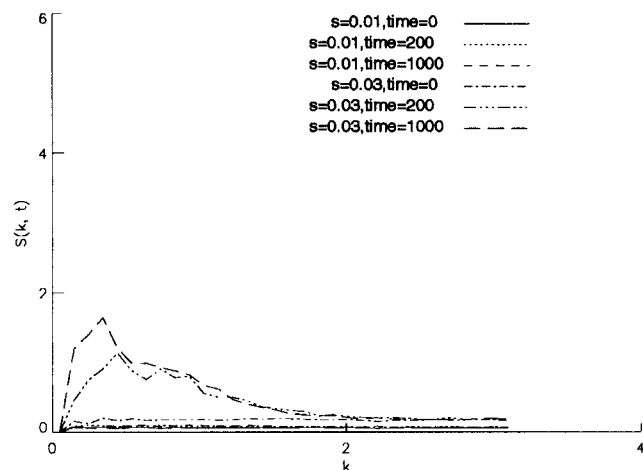
Figure 1. Temporal evolution of surfactant density structure function S(k,t) for binary water and surfactant mixtures. The figure contains results for both s = 0.01 and s = 0.03 reduced density of surfactant.
