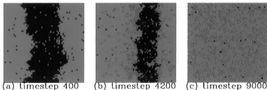
Figure 4. Three snapshots in time from the evolution of the lattice-gas automaton simulation of Figure 3. Oily ester molecules are black, water is red, and surfactant is green.
