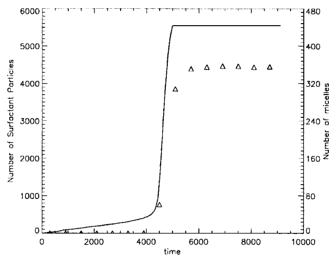
Figure 3. Amphiphile and micelle concentration as a function of the time step in the lattice-gas automaton model. The triangles are for the micelles and correspond to the values indicated on the right hand vertical axis.
